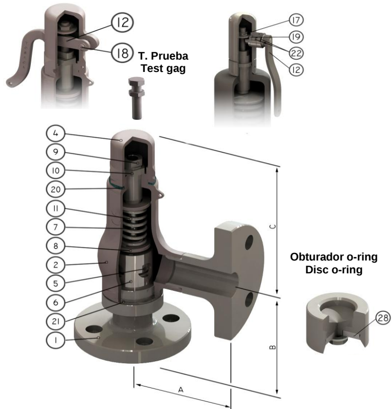
Palanca manual Lifting device
